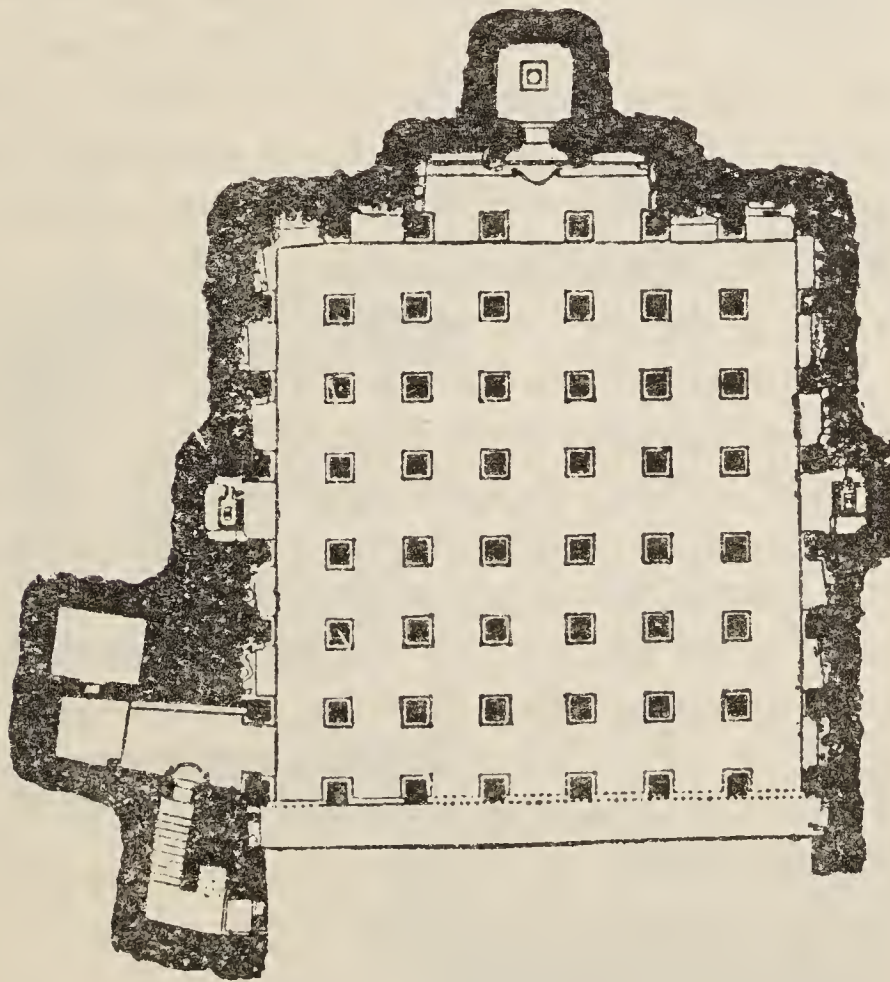
Fig. 13. Ellora, Daśāvatāra Cave: Plan of upper storey.
