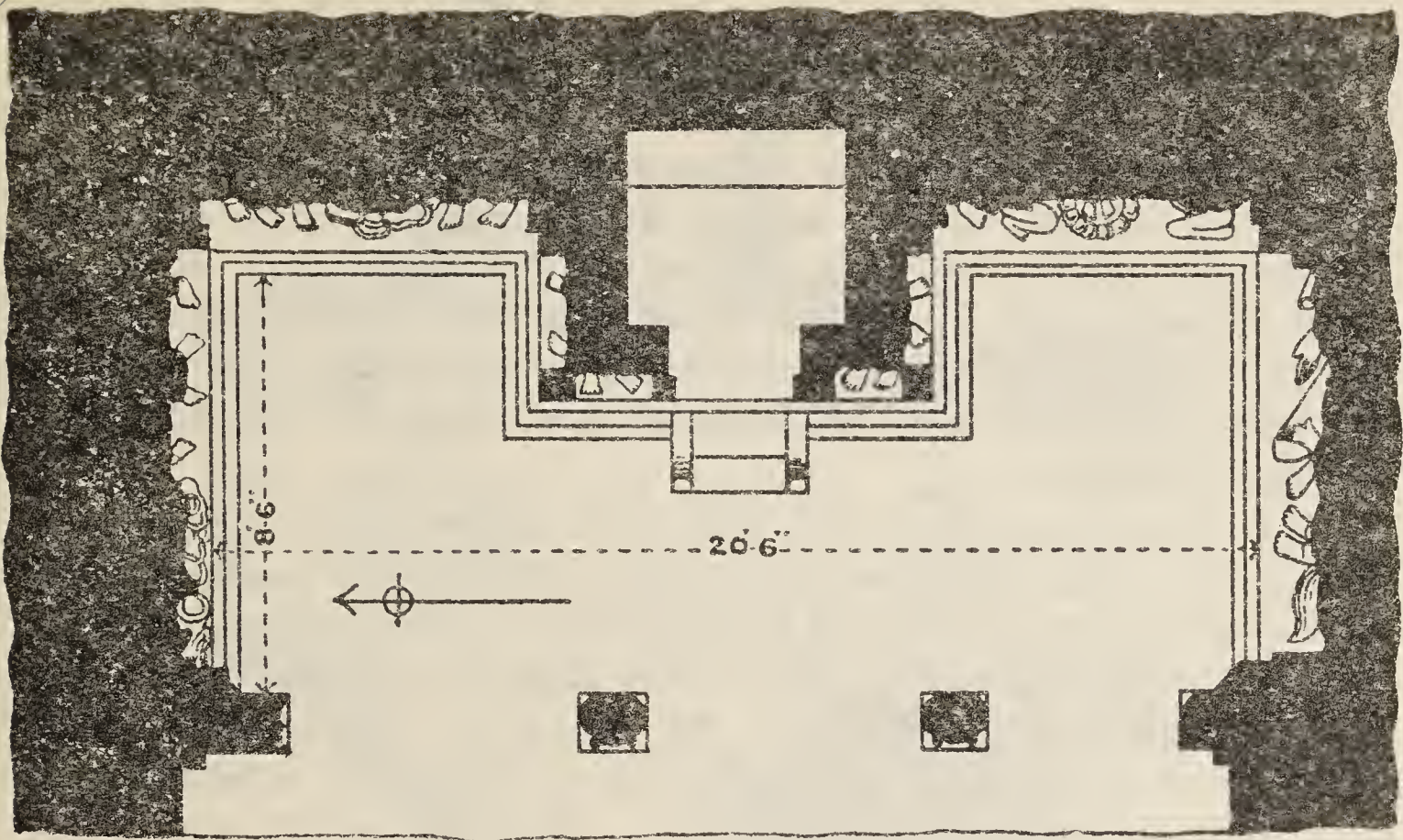
Fig. 12. Māmallapuram, Varāha-maṇḍapa: Plan.
