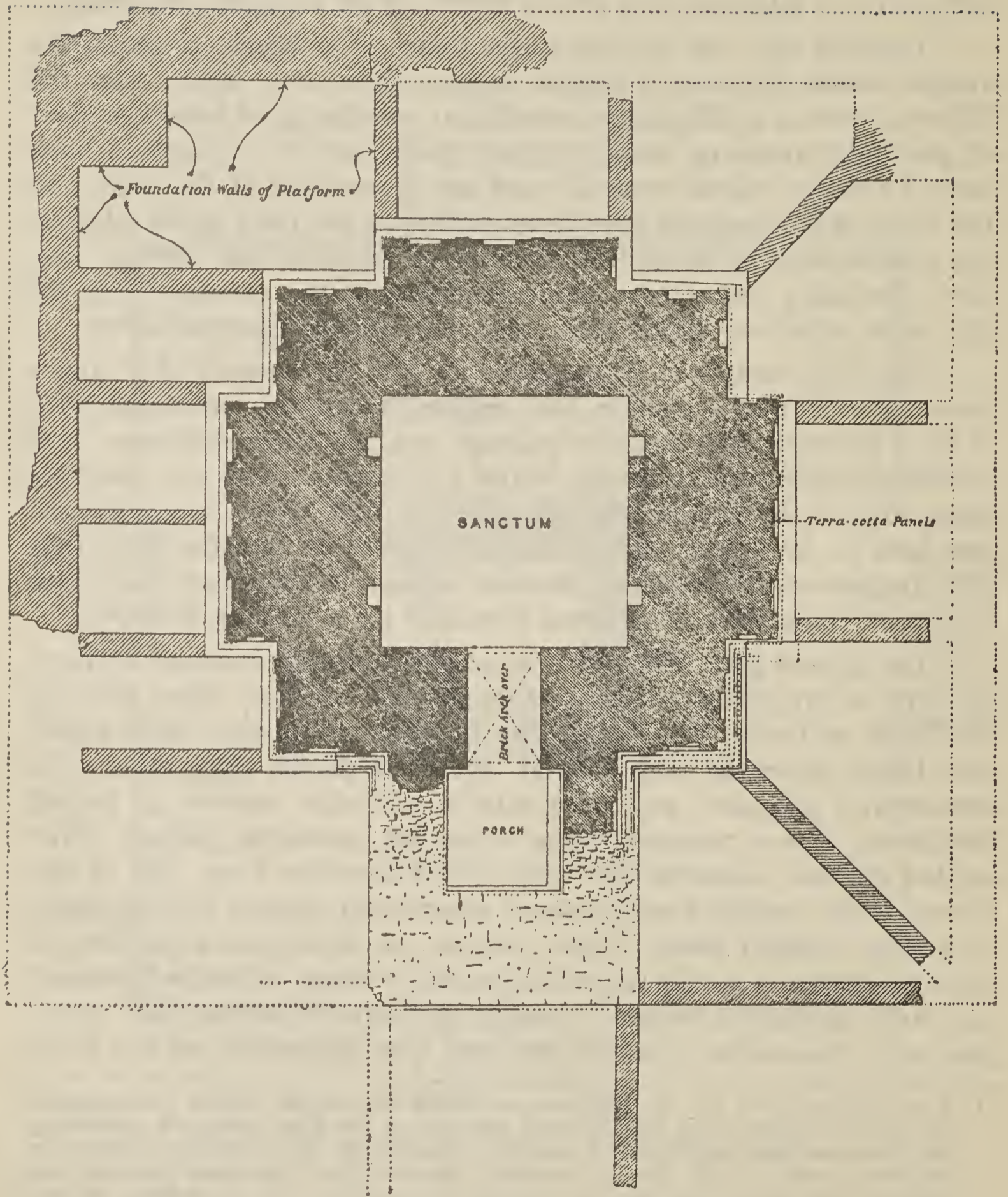
Fig. 26. Bhitargāon, Brick temple: Plan.
