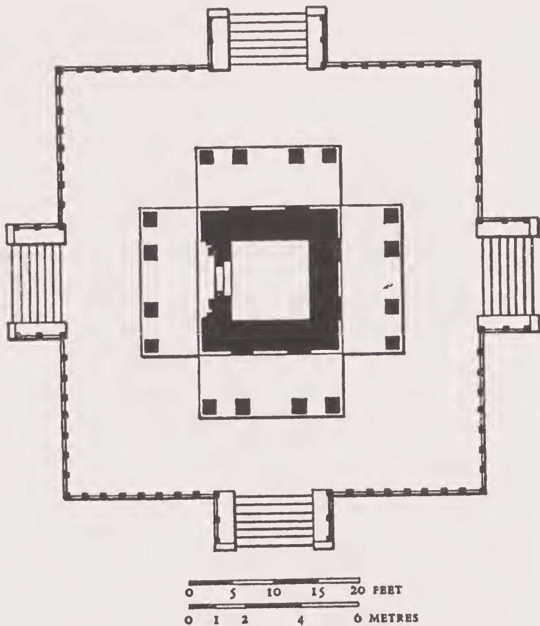
4. Vishnu temple, Deogarh: plan
